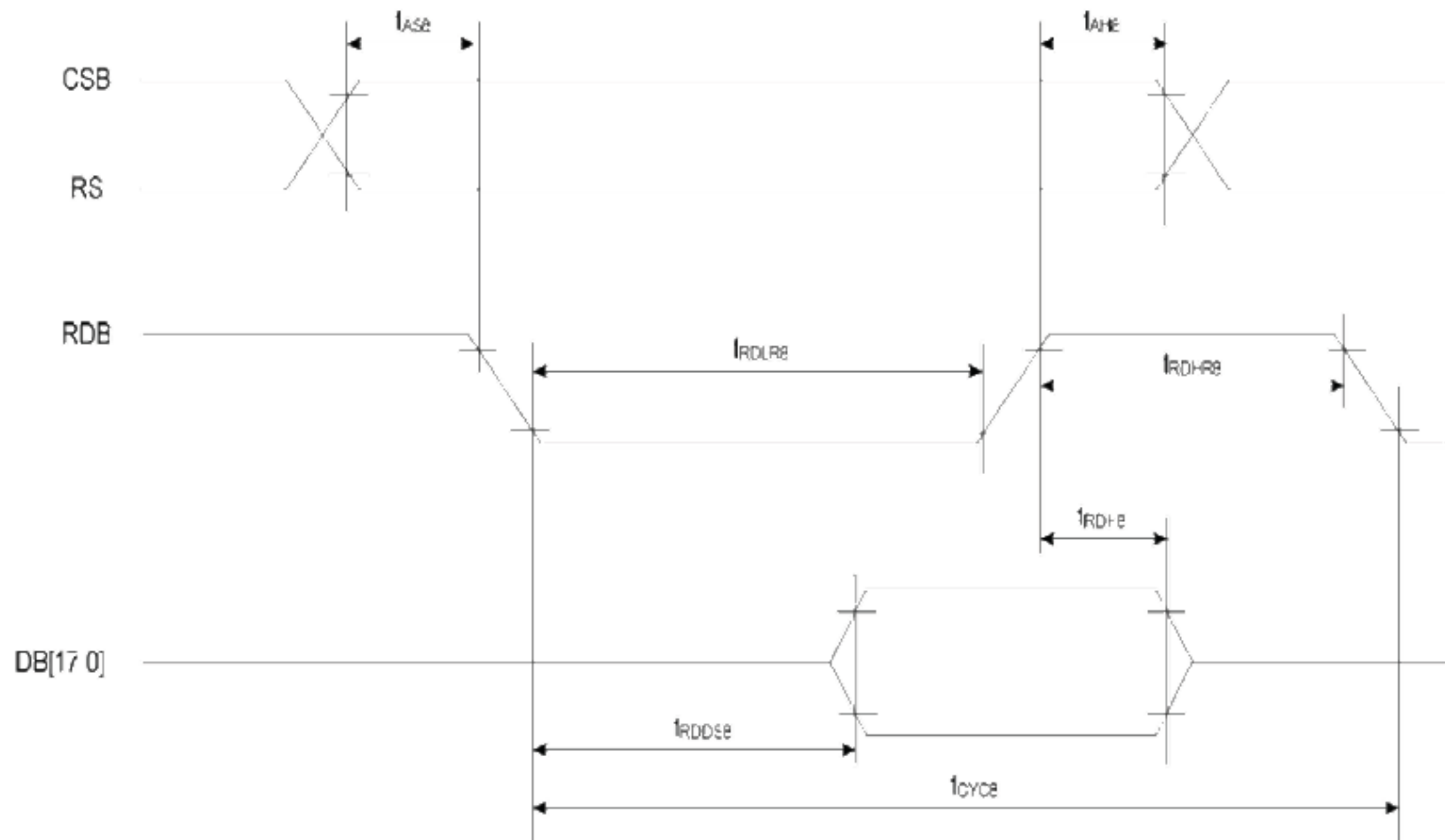
( Read Timing )
