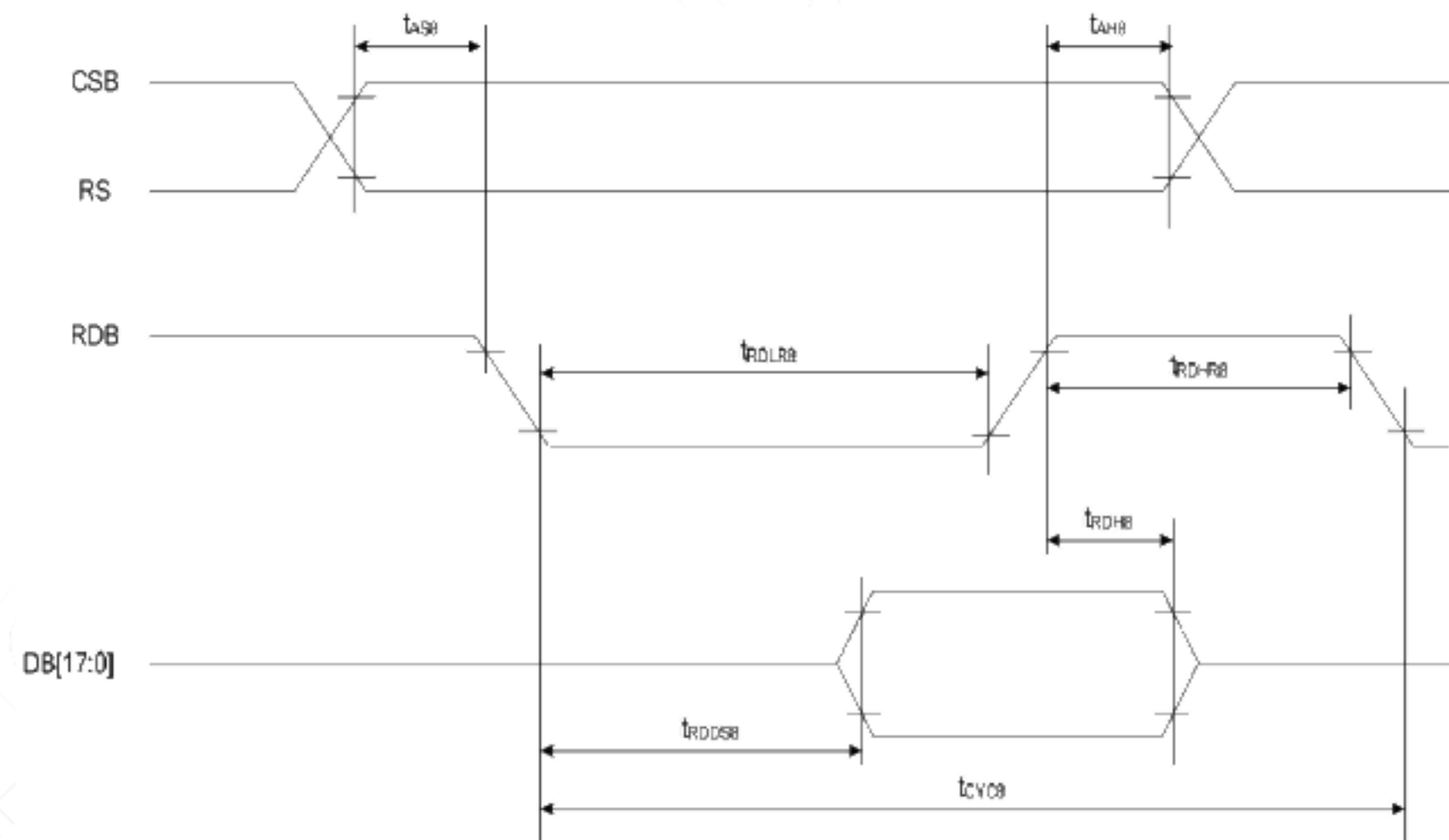
( Read Timing )
