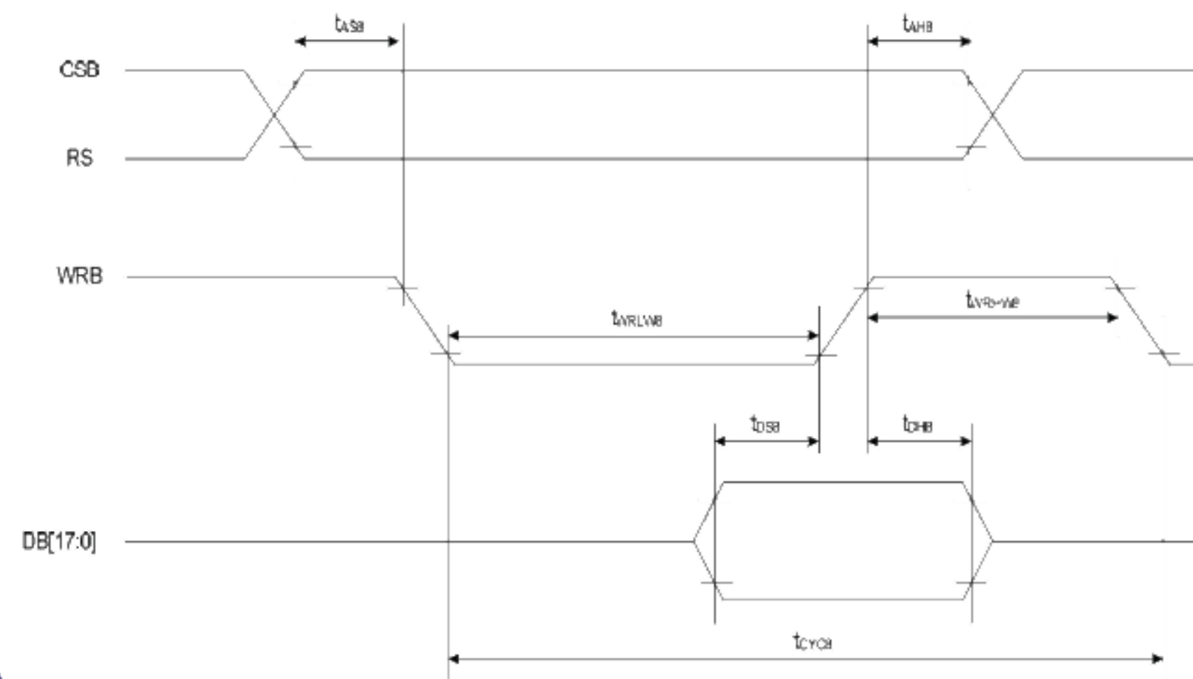
( Write Timing )
