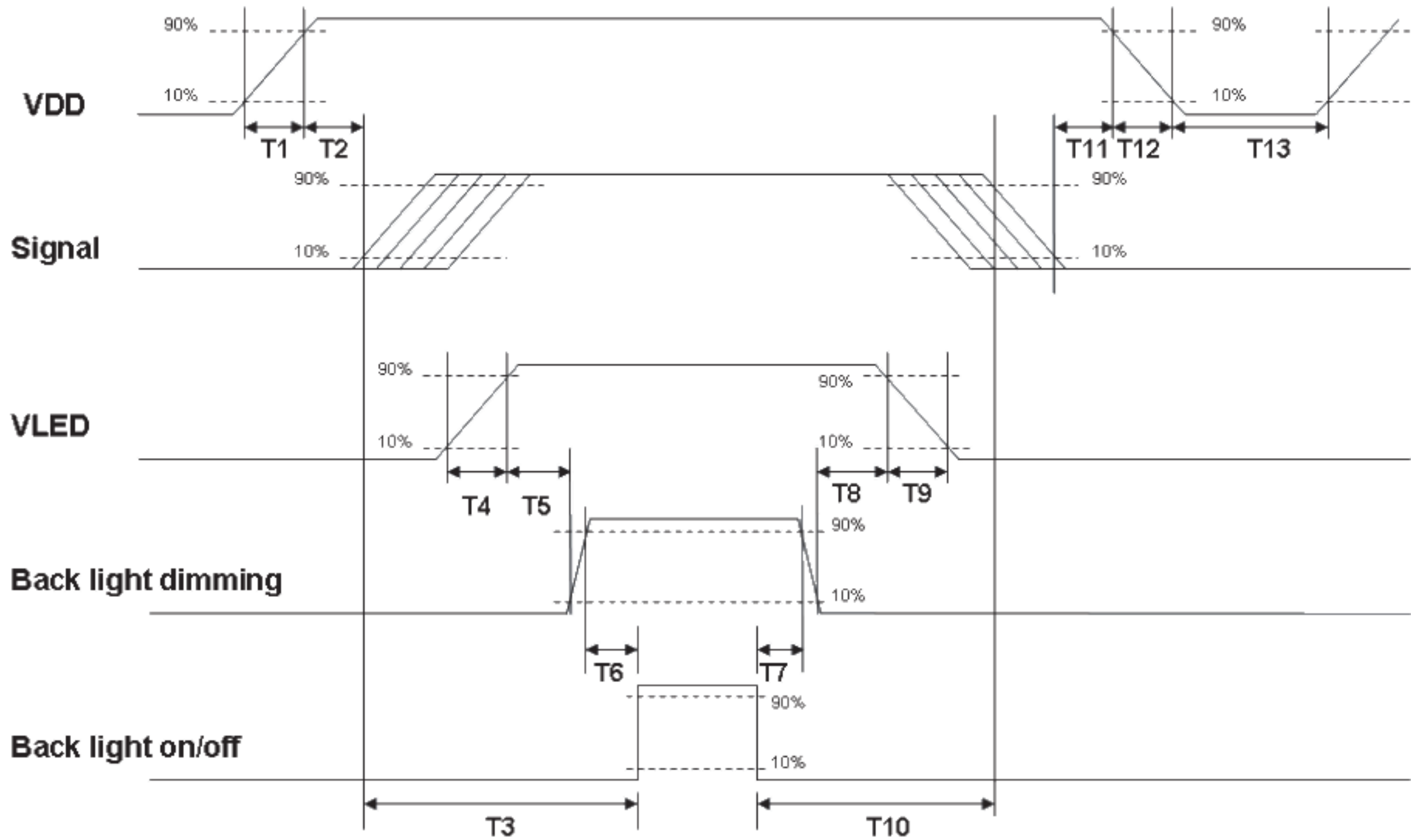
Power sequence timing
