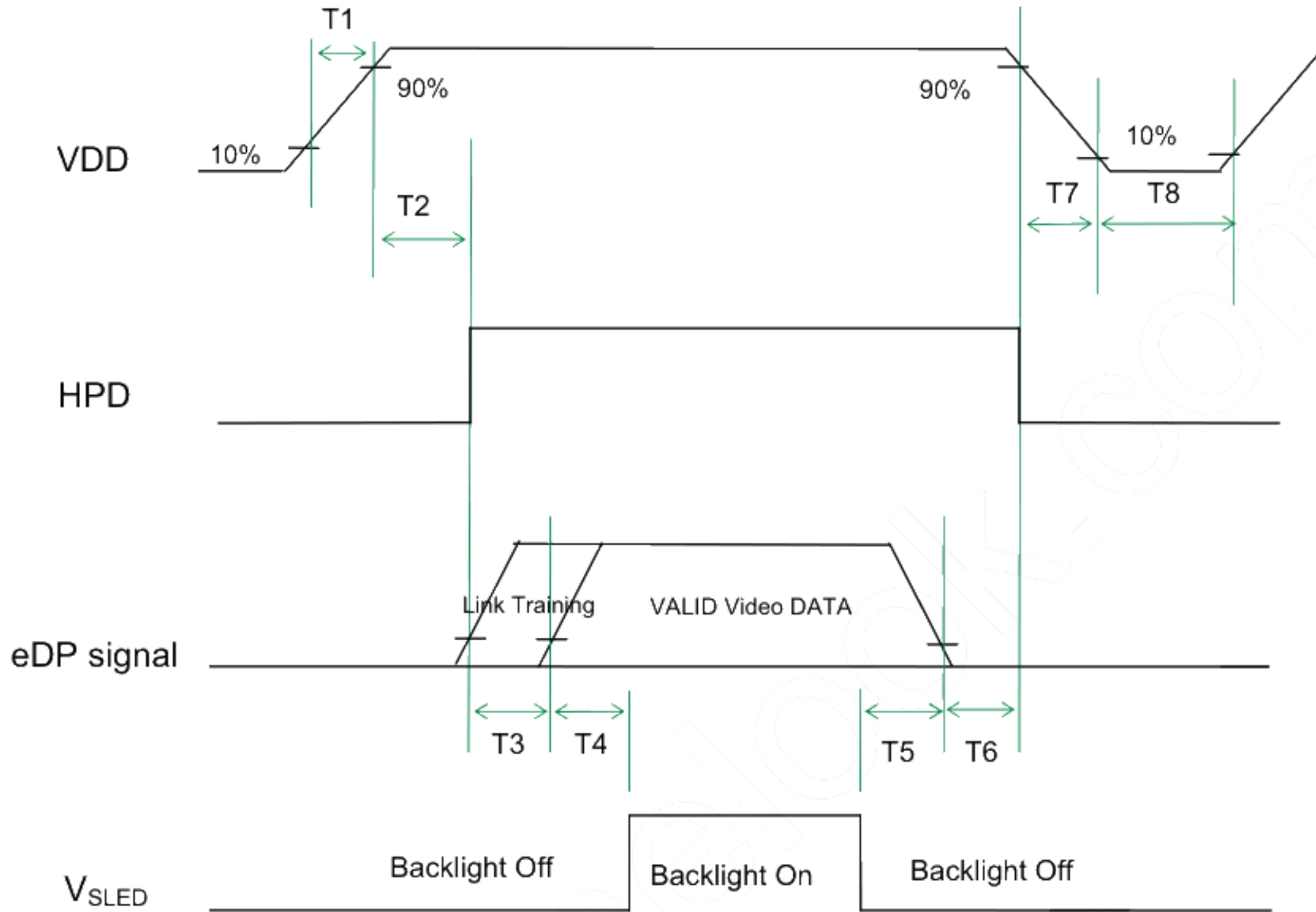
Power ON/OFF sequence timing
