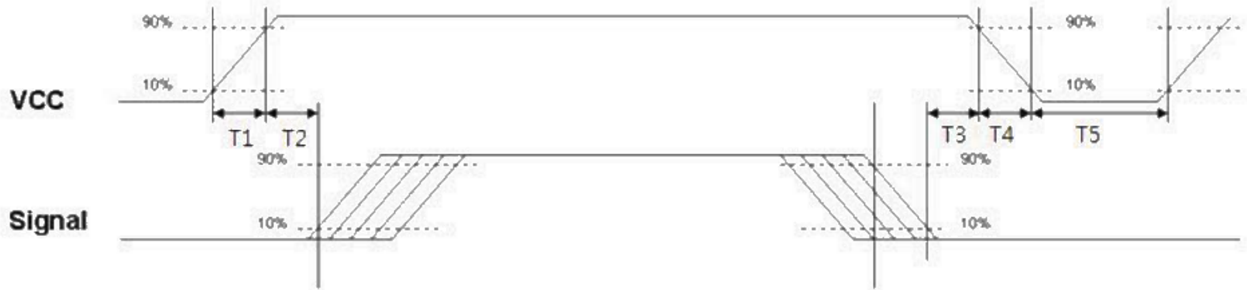
Power Sequence Timing
