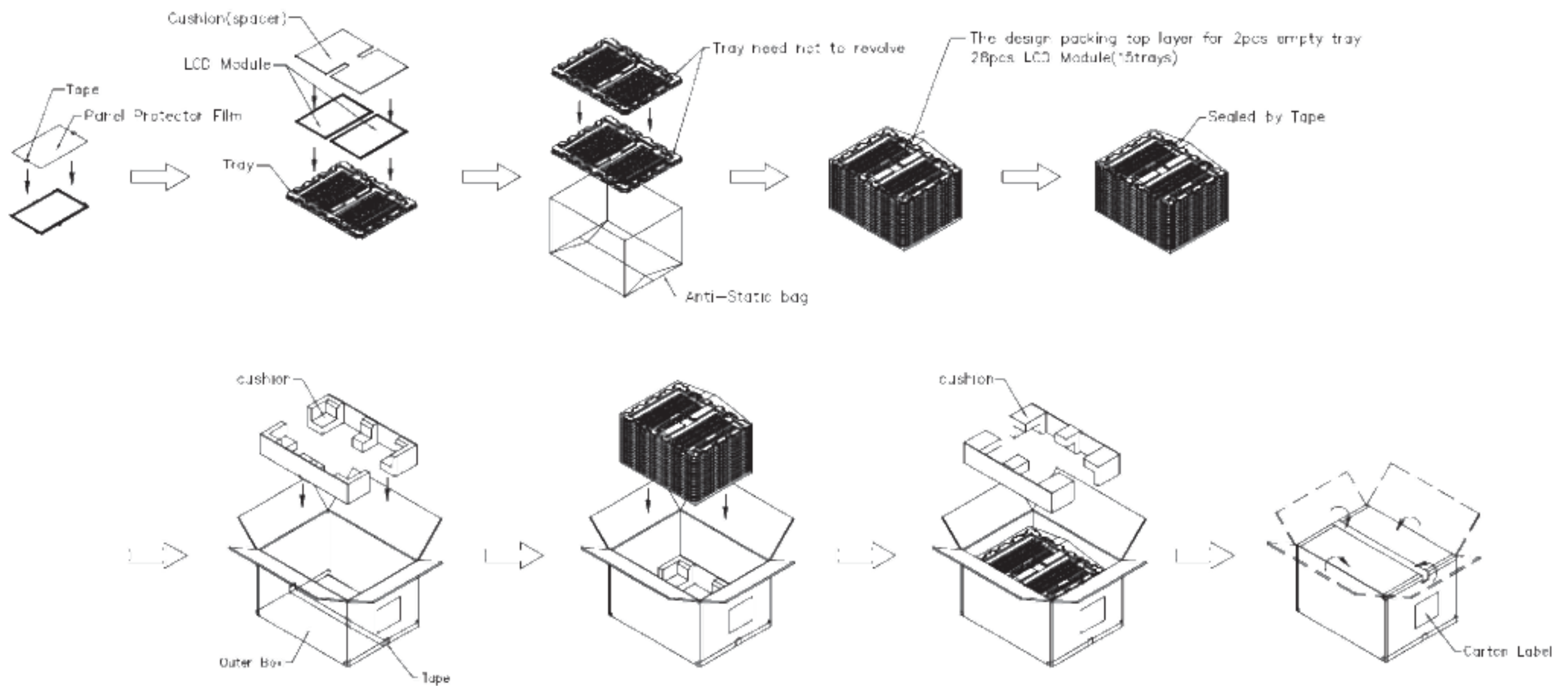
Figure. 9-1 Packing method
