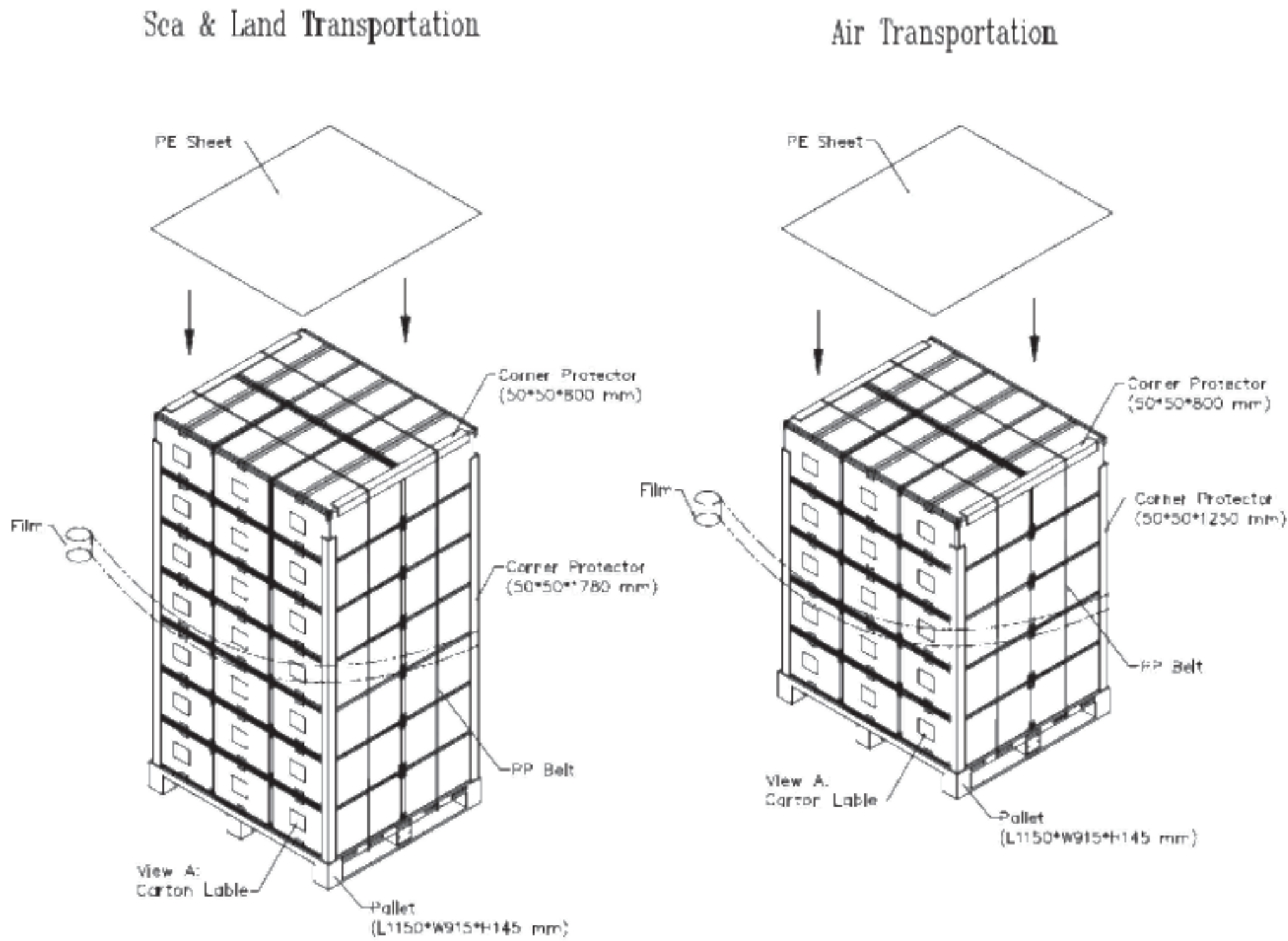
Figure. 9-2 Packing method
